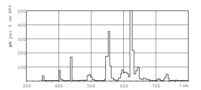
LDPB_TL5-HE8_827-Spectral power distribution B/W
