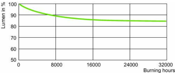
Lumen Maintenance Diagram - MASTER GreenPower Plus 600W EL E40 1SL
