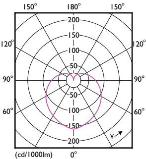
Light Distribution Diagram - CorePro LEDbulb ND 4.9-40W A60 E27 940
