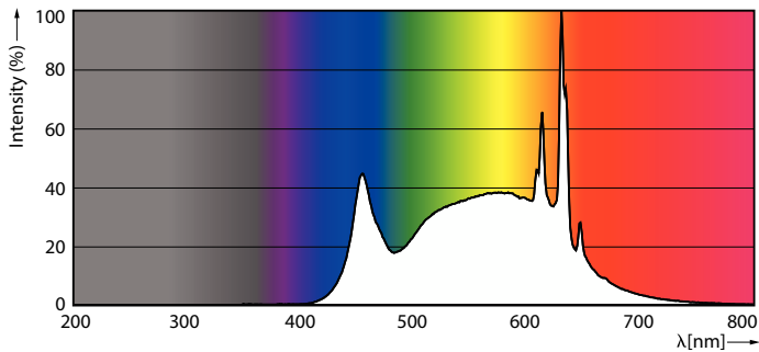
Spectral Power Distribution Colour - CorePro LEDbulb ND 4.9-40W A60 E27 940
