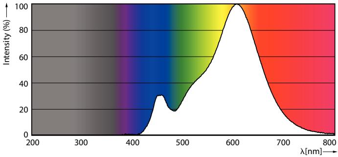
Spectral Power Distribution Colour - CorePro LEDbulb ND 4.9-40W A60 B22 827
