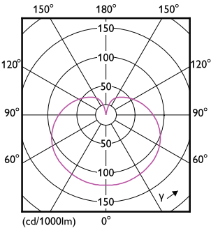
Light Distribution Diagram - CorePro LEDbulb ND 4.9-40W A60 B22 827
