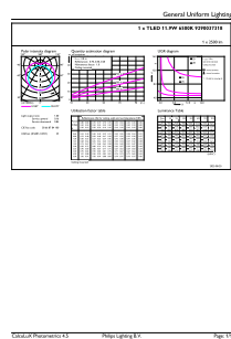
General uniform lighting - MAS LEDtube 1200mm UE 11.9W 865 T8 EELA
