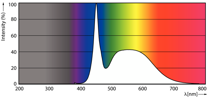
Spectral Power Distribution Colour - LEDtube Connected IA 1500mm 23.1W865 T8
