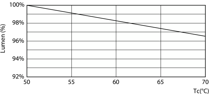
Lumen Maintenance Diagram - LEDtube Connected IA 1500mm 23.1W865 T8
