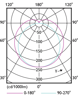
Light Distribution Diagram - LEDtube Connected IA 1500mm 23.1W865 T8
